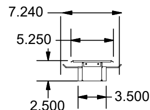
4' 3"W H25, End View
