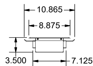
4' 6"W H25, End View
